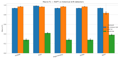
Fig. 5. Historical detector comparison. ADWIN, Page-Hinkley and EDMA never fire and therefore reproduce the frozen baseline exactly; EDD fires most often and reaches the highest macro-F1 at the highest adaptation cost, while RAPT adapts least among the methods that adapt at all.
